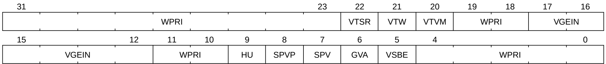
Figure 69. Hypervisor status register ( hstatus ) when HSXLEN=32
