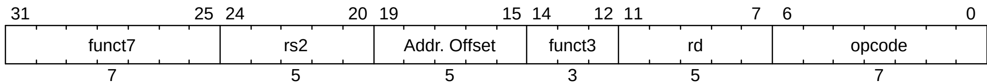
Figure 77. Transformed virtual-machine load/store instruction (HLV, HLVX, HSV). All fields are the same as the trapping instruction except bits 19:15, Addr. Offset
