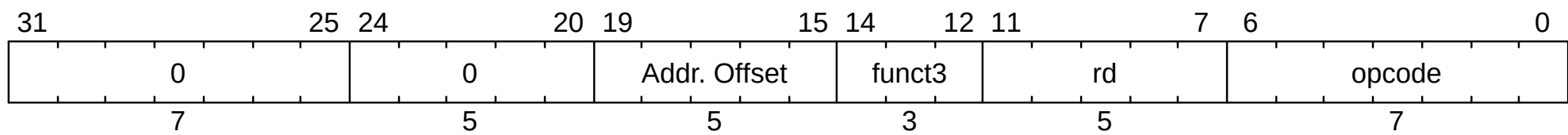
Figure 74. Transformed load instruction (LB, LBU, LH, LHU, LW, LWU, LD, FLW, FLD, FLQ, or FLH). Fields funct3 , rd , and opcode are the same as the trapping load instruction.
