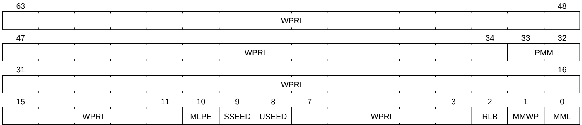
Figure 52. Machine security configuration ( mseccfg ) register.
