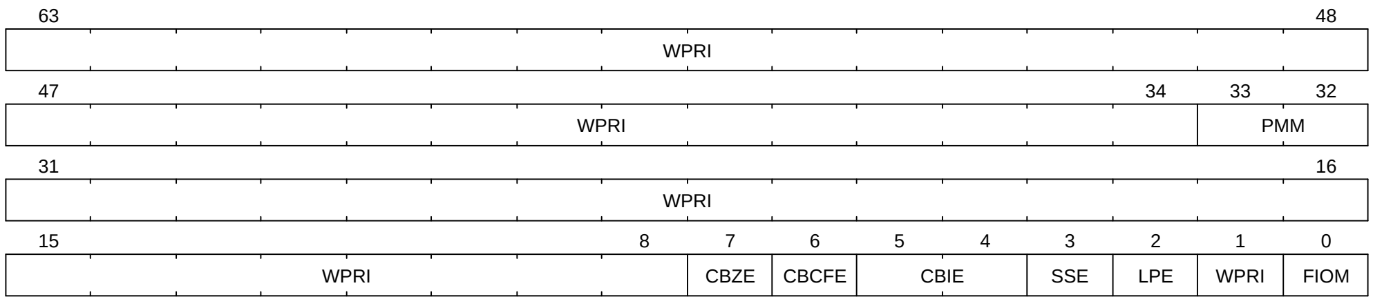
Figure 65. Supervisor environment configuration register ( senvcfg ) for RV64.
