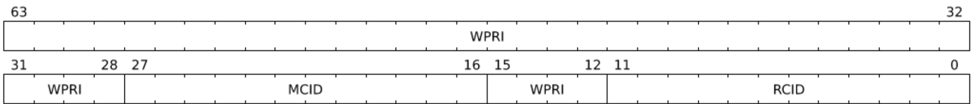
Figure 67. Supervisor Resource Management Configuration ( srmcfg ) register for SXLEN =64
