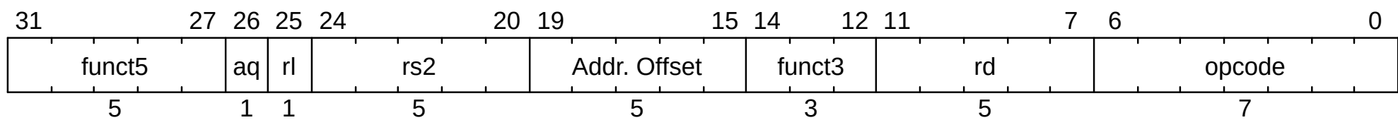
Figure 76. Transformed atomic instruction (load-reserved, store-conditional, or AMO instruction). All fields are the same as the trapping instruction except bits 19:15, Addr. Offset .
