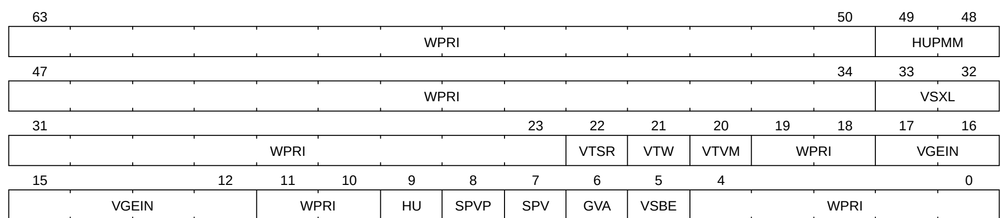
Figure 70. Hypervisor status register ( hstatus ) when HSXLEN =64.
