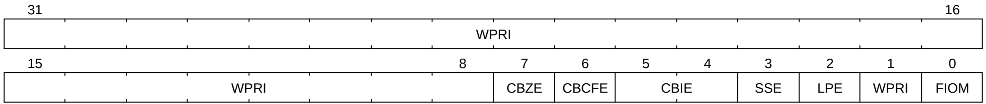
Figure 66. Supervisor environment configuration register ( senvcfg ) for RV32.
