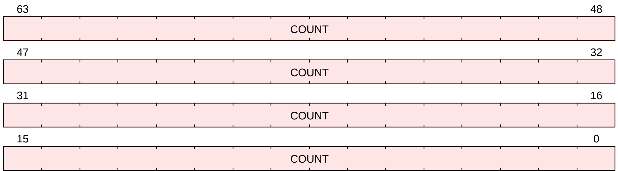
Figure 29. hpmcounter4 format
