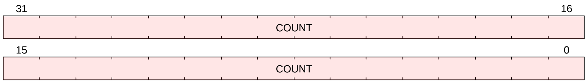
Figure 42. timeh format
