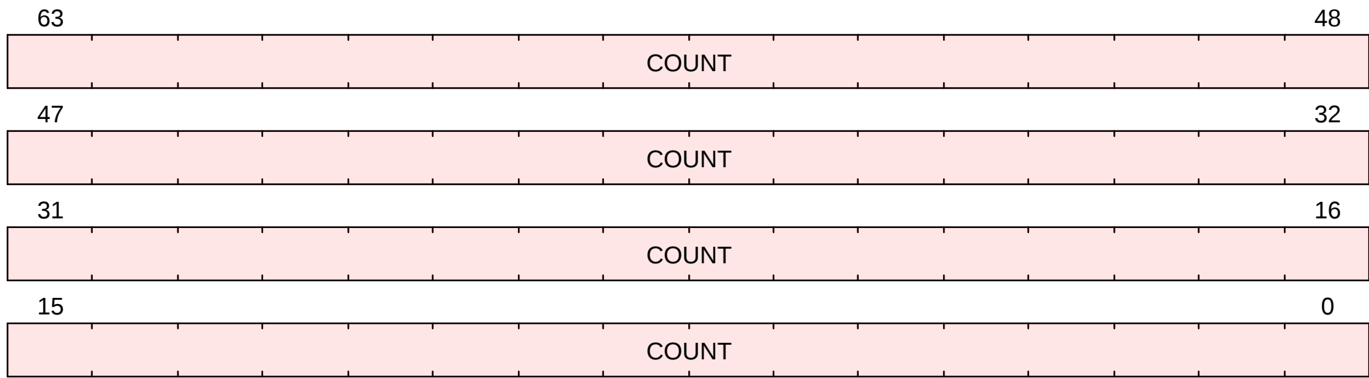
Figure 12. hpmcounter16 format
