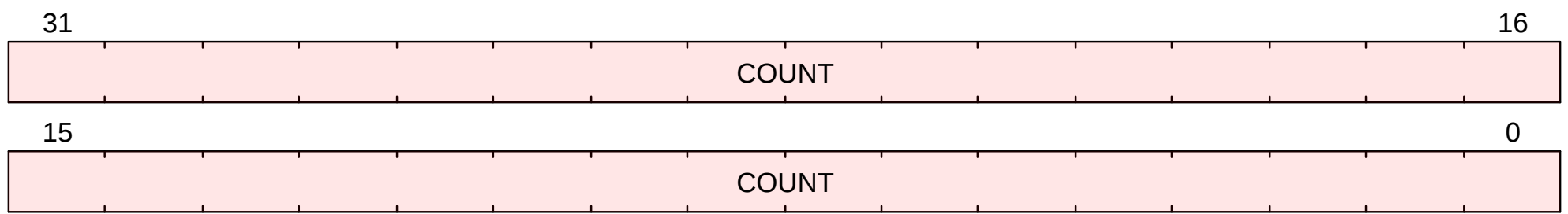
Figure 40. minstreth format
