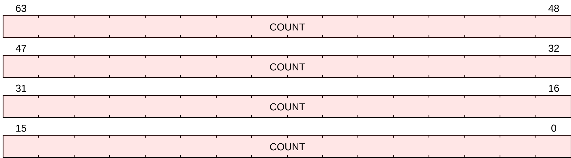
Figure 31. hpmcounter6 format
