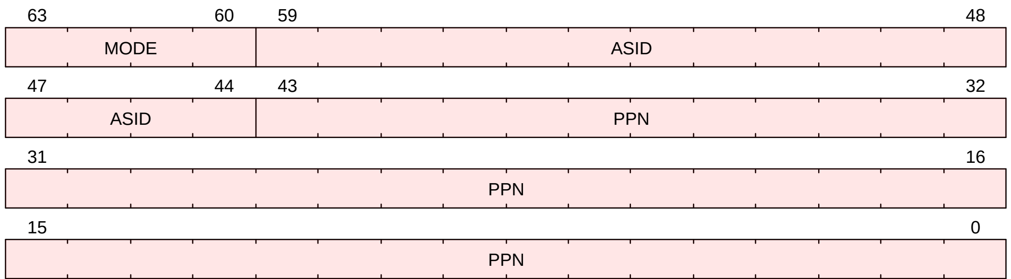
Figure 56. satp Format when CSR[mstatus].SXL == 1
