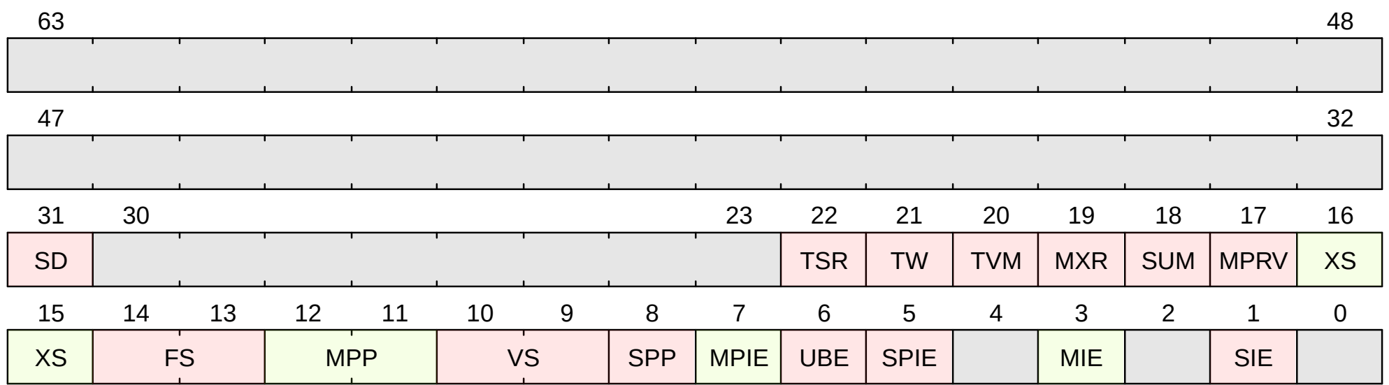
Figure 51. mstatus format
