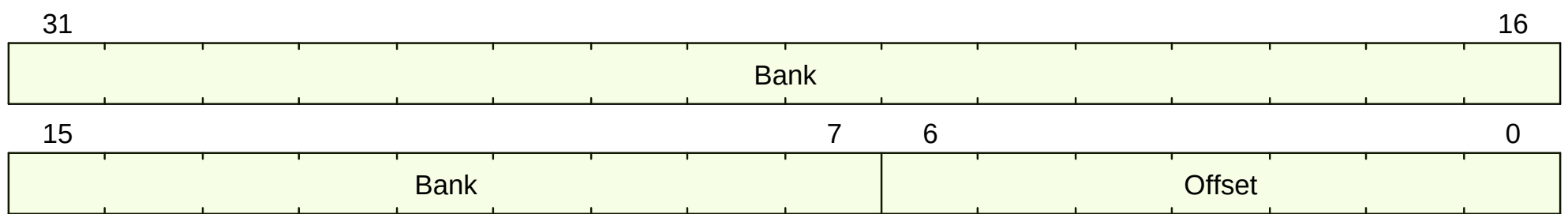
Figure 54. mvendorid format
