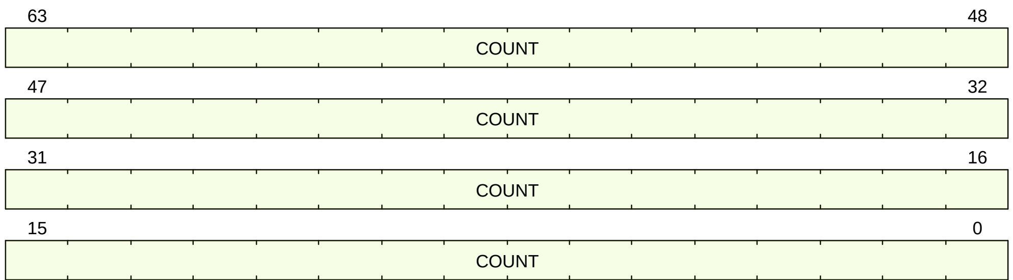
Figure 45. minstret format
