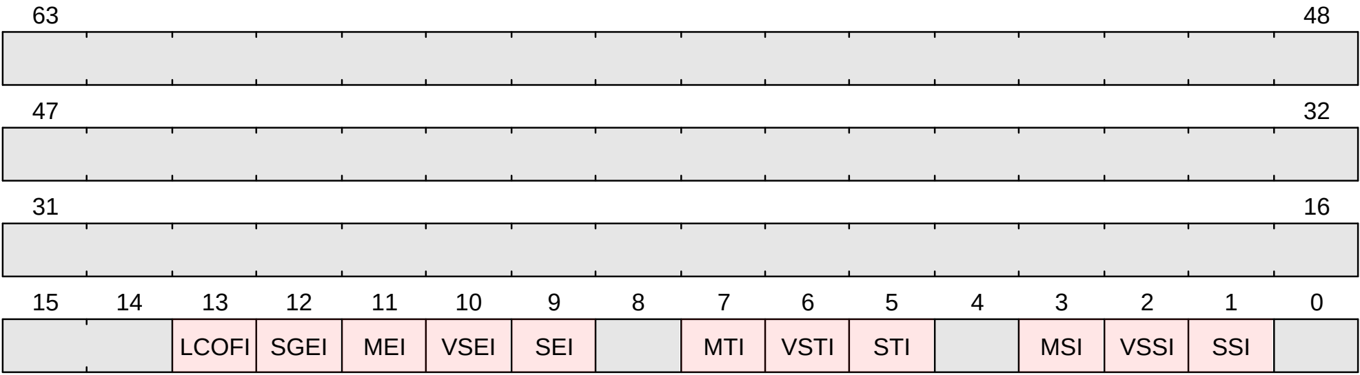
Figure 42. mideleg format
