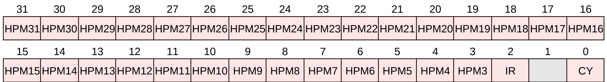
Figure 36. mcountinhibit format
