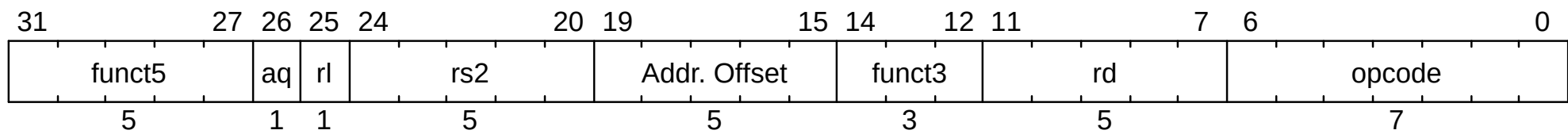
Figure 101. Transformed atomic instruction (load-reserved, store-conditional, or AMO instruction). All fields are the same as the trapping instruction except bits 19:15, Addr. Offset .
