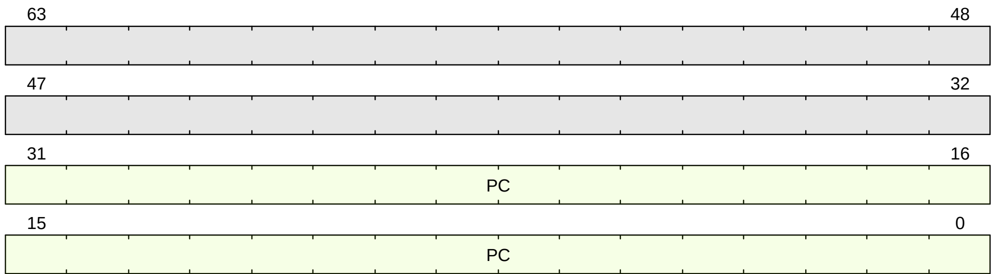
Figure 40. mepc format
