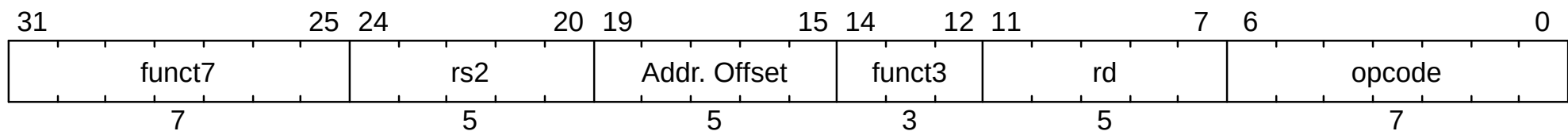
Figure 102. Transformed virtual-machine load/store instruction (HLV, HLVX, HSV). All fields are the same as the trapping instruction except bits 19:15, Addr. Offset
