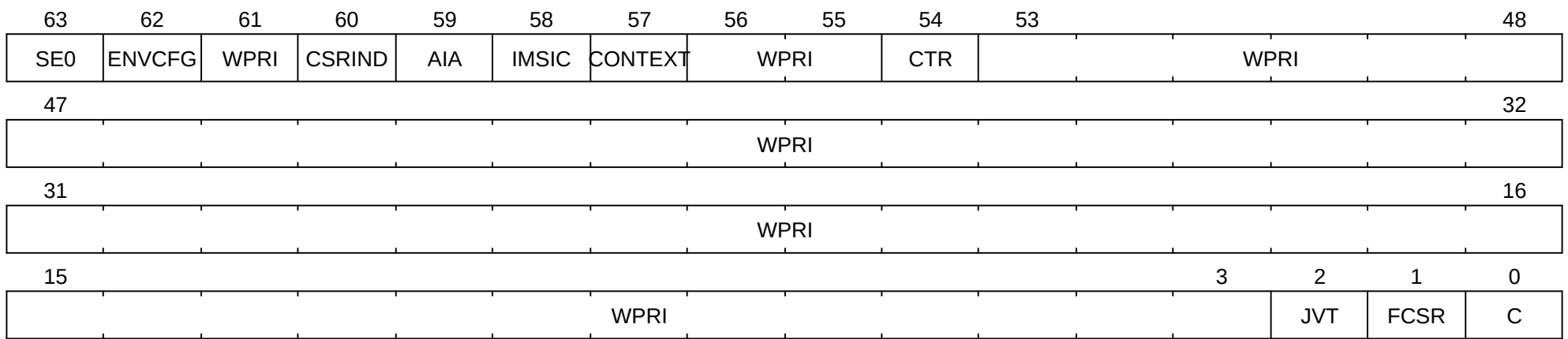
Figure 81. Hypervisor State Enable 0 Register (hstateen0)
