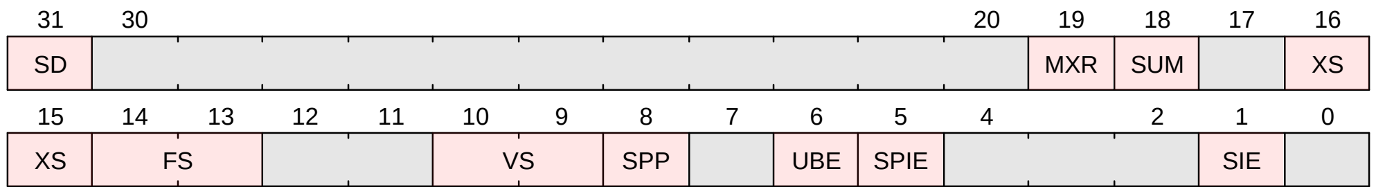
Figure 64. sstatus Format when CSR[mstatus].SXL == 0
