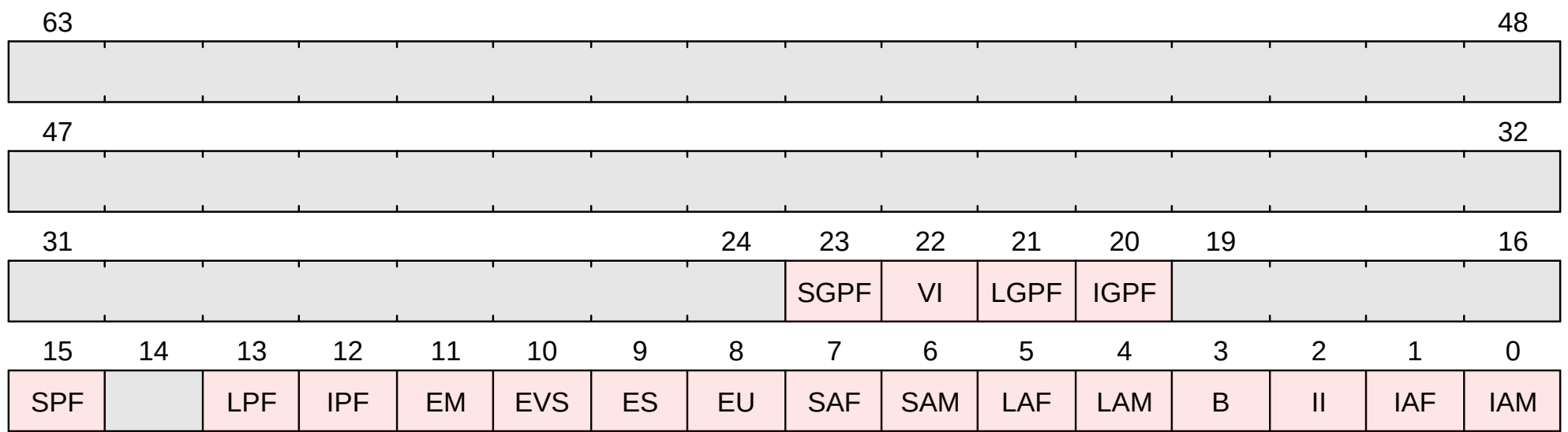
Figure 39. medeleg format
