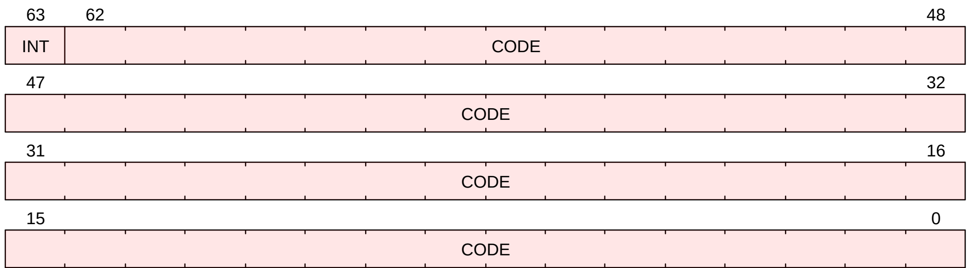
Figure 58. scause Format when CSR[mstatus].SXL == 1
