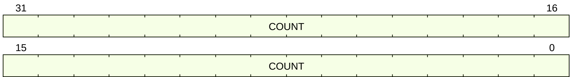
Figure 2. cycleh format
