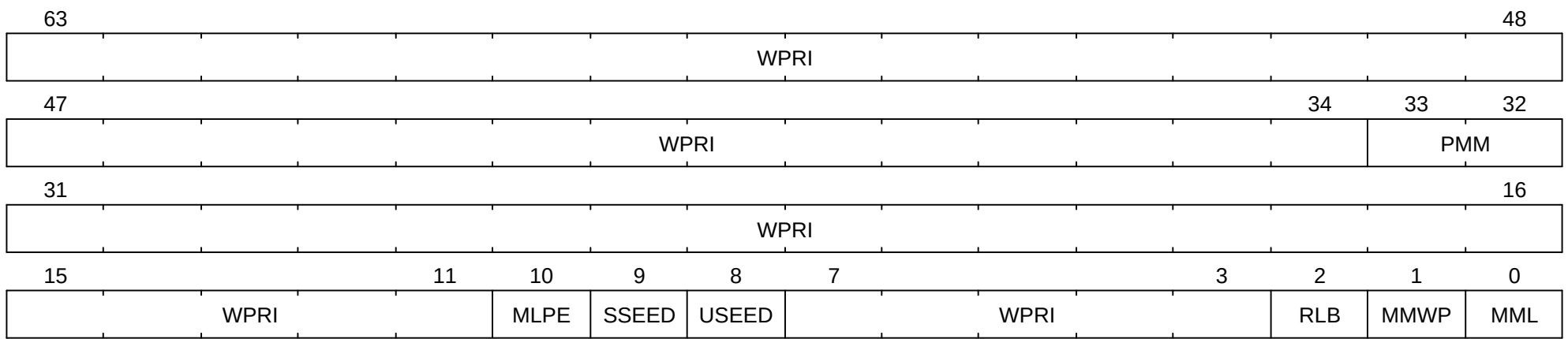
Figure 79. Machine security configuration ( mseccfg ) register.
