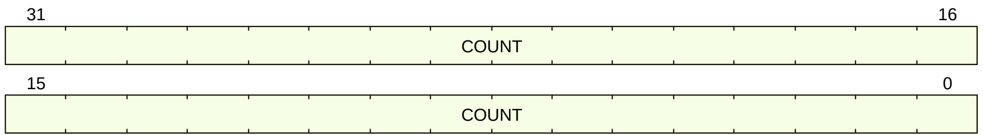
Figure 69. timeh format
