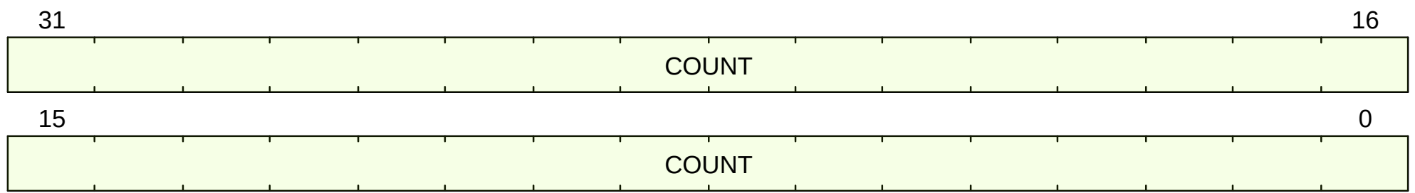
Figure 46. minstreth format
