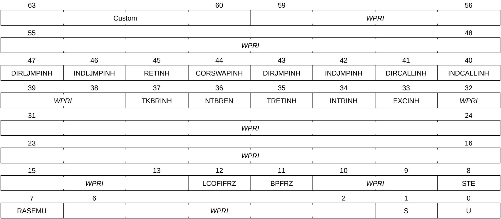
Figure 84. Virtual Supervisor Control Transfer Records Control Register Format
