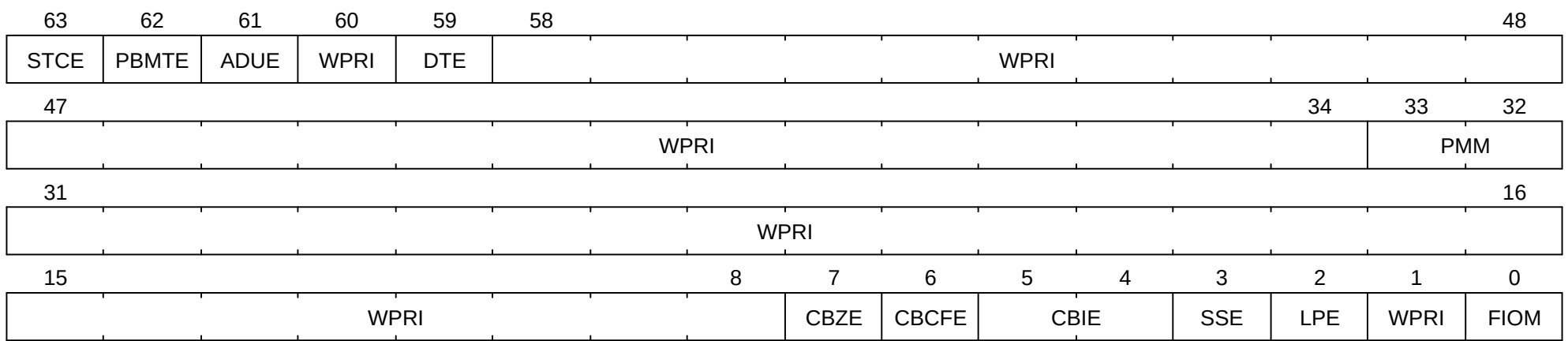
Figure 96. Hypervisor environment configuration register ( henvcfg ).
