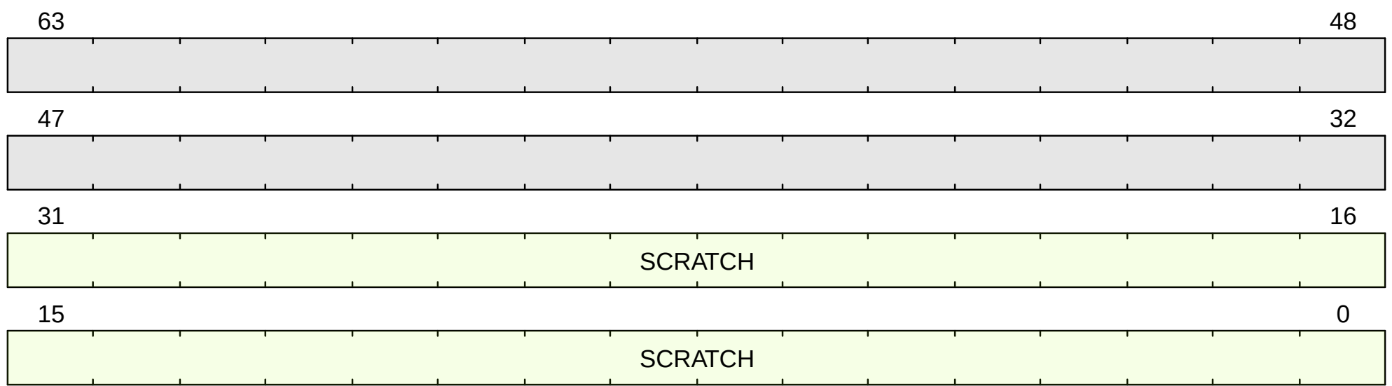
Figure 50. mscratch format
