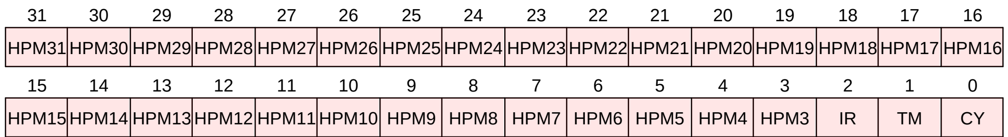
Figure 59. scounteren format
