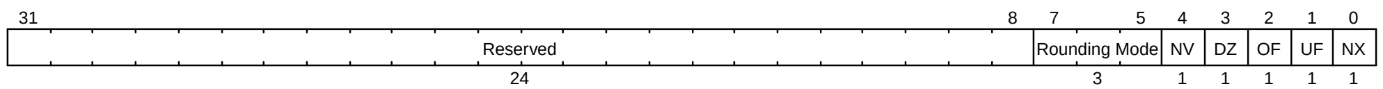
Figure 71. Floating-point control and status register
