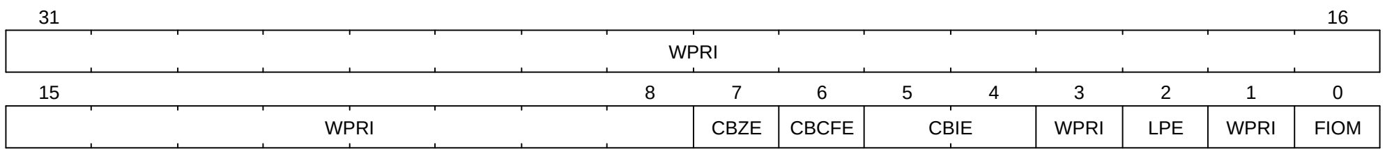
Figure 93. Supervisor environment configuration register ( senvcfg ) for RV32.
