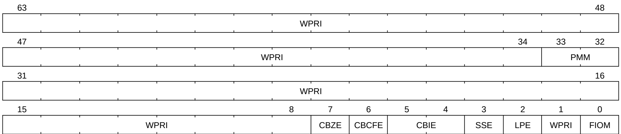
Figure 92. Supervisor environment configuration register ( senvcfg ) for RV64.
