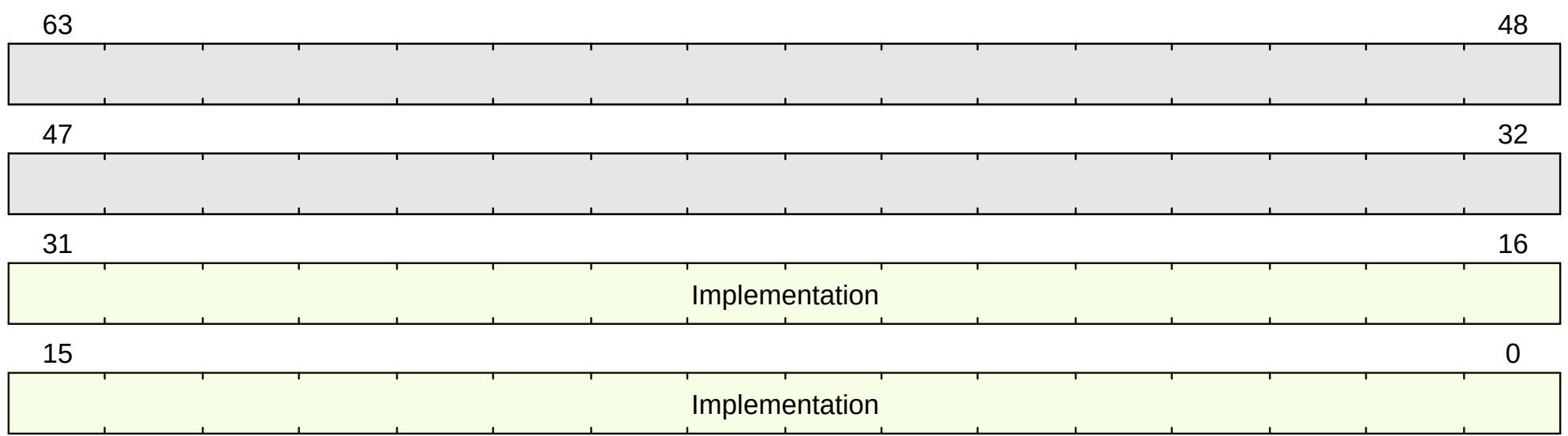
Figure 44. mimpid format
