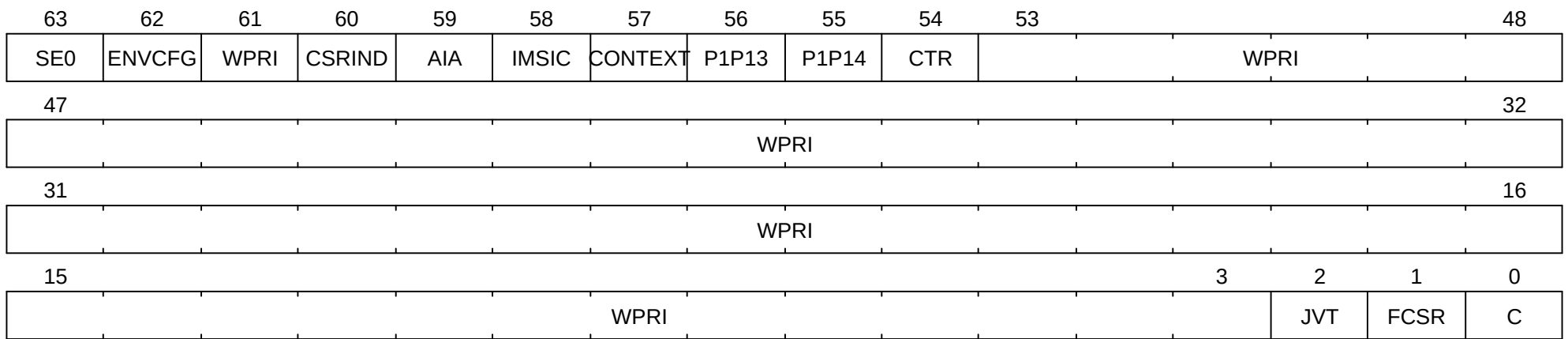
Figure 80. Machine State Enable 0 Register (mstateen0)
