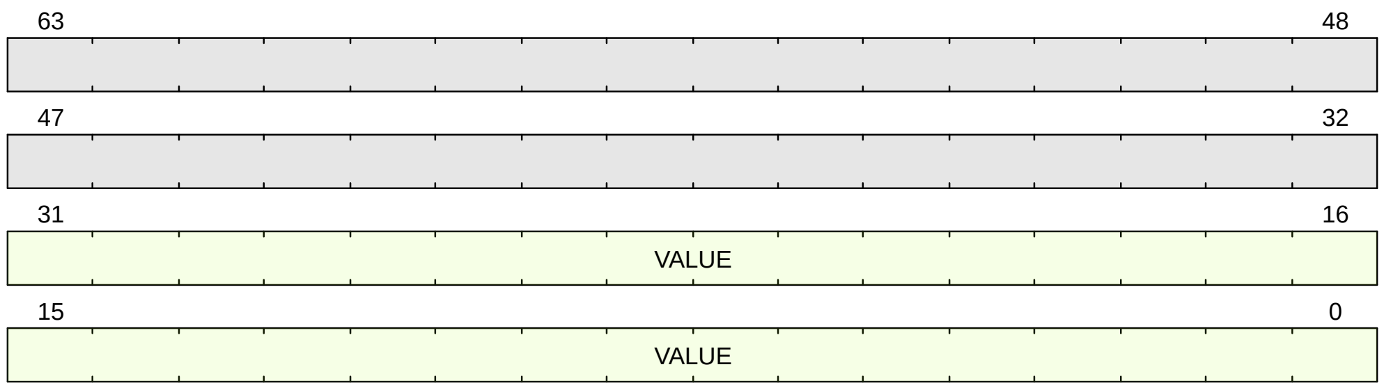
Figure 52. mtval format
