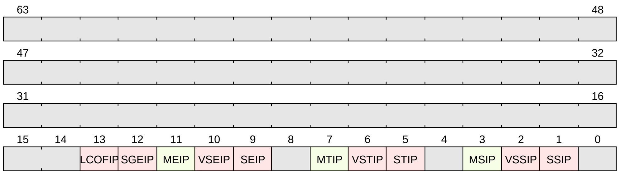
Figure 47. mip format
