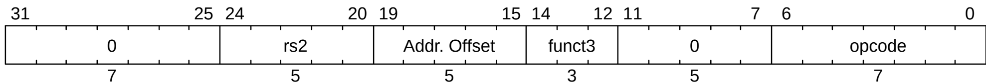
Figure 100. Transformed noncompressed store instruction (SB, SH, SW, SD, FSW, FSD, FSQ, or FSH). Fields rs2 , funct3 , and opcode are the same as the trapping store instruction.
