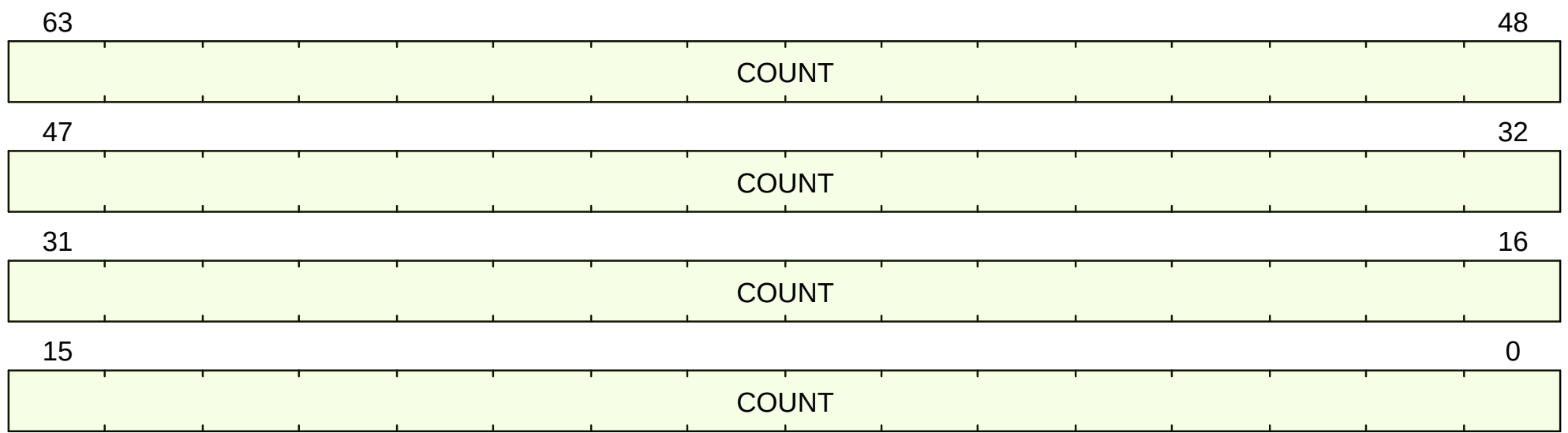
Figure 32. instret format
