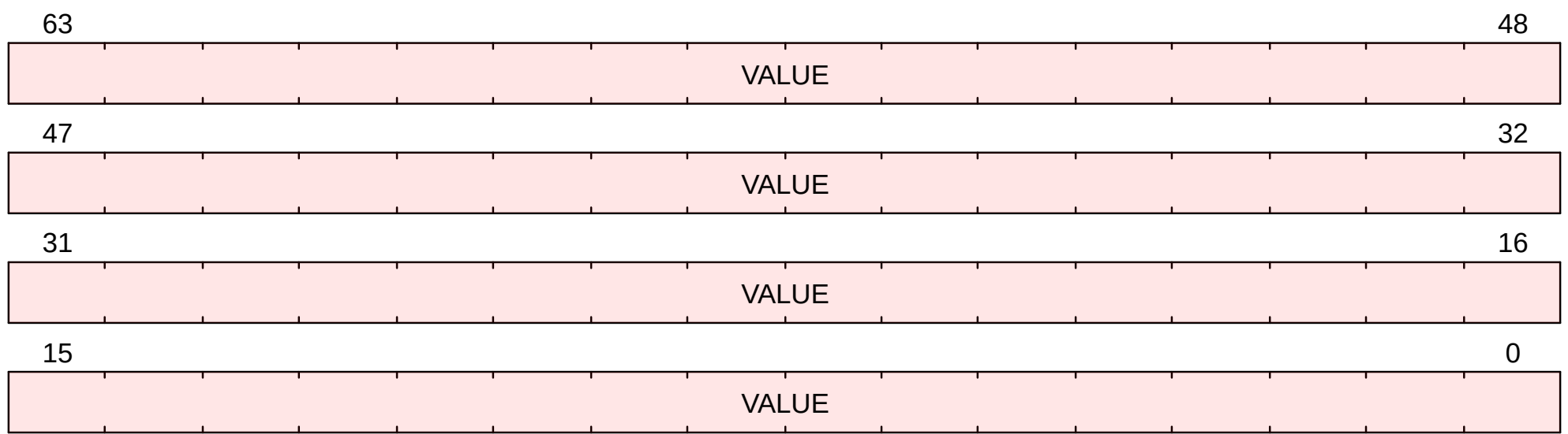
Figure 66. stval format
