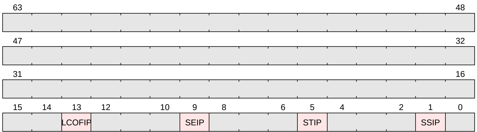
Figure 62. sip format
