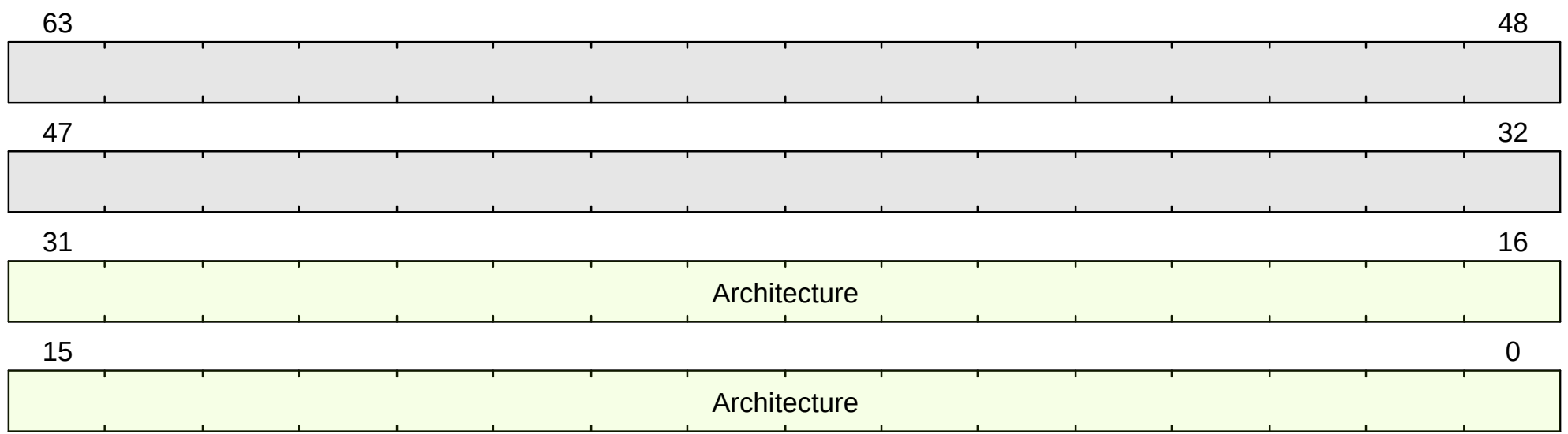
Figure 34. marchid format
