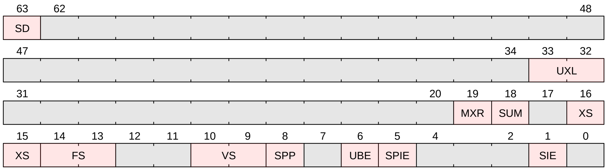
Figure 65. sstatus Format when CSR[mstatus].SXL == 1
