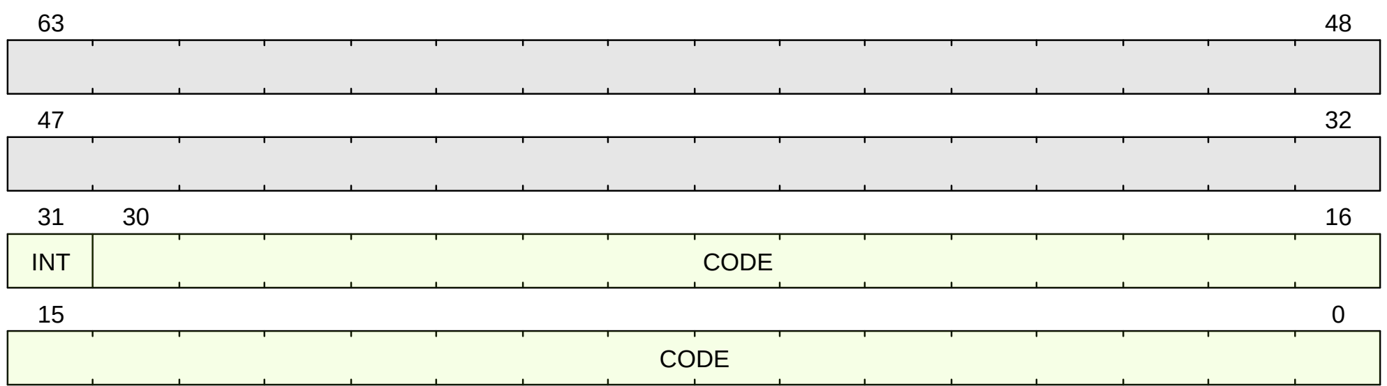
Figure 35. mcause format
