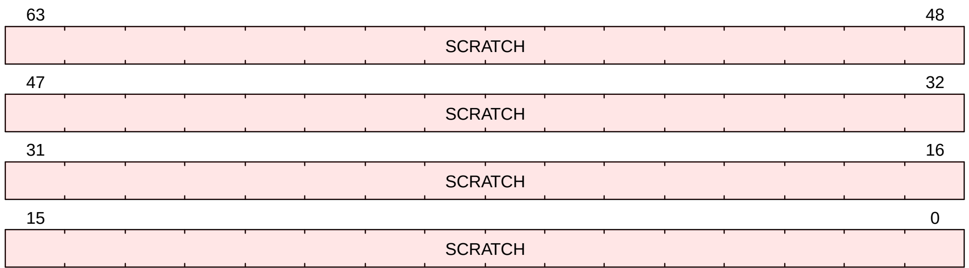
Figure 63. sscratch format
