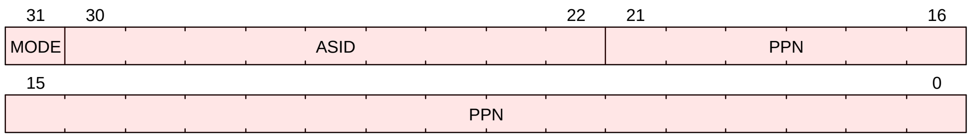
Figure 55. satp Format when CSR[mstatus].SXL == 0
