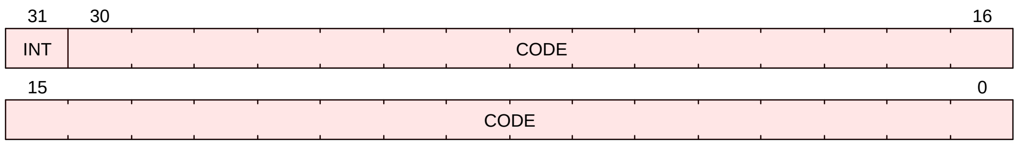
Figure 57. scause Format when CSR[mstatus].SXL == 0
