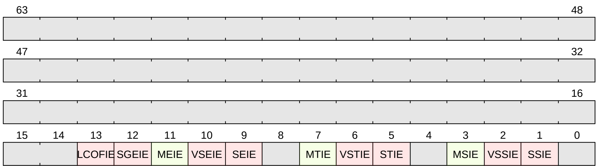
Figure 43. mie format
