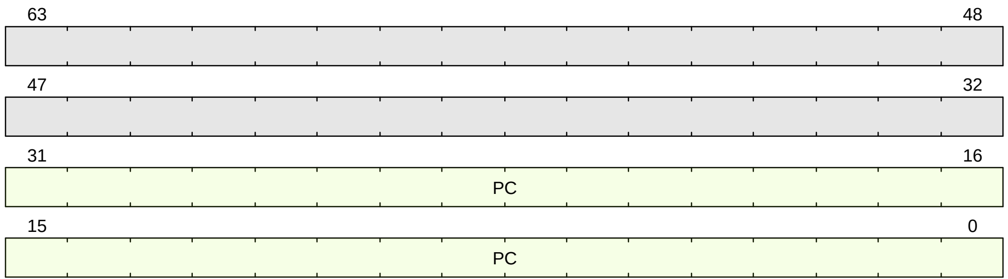
Figure 49. mnepc format
