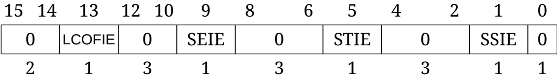
Figure 136. Standard portion (bits 15:0) of vsie .
