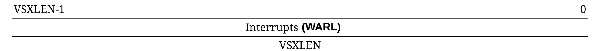
Figure 133. Virtual supervisor interrupt-pending register ( vsip ).
