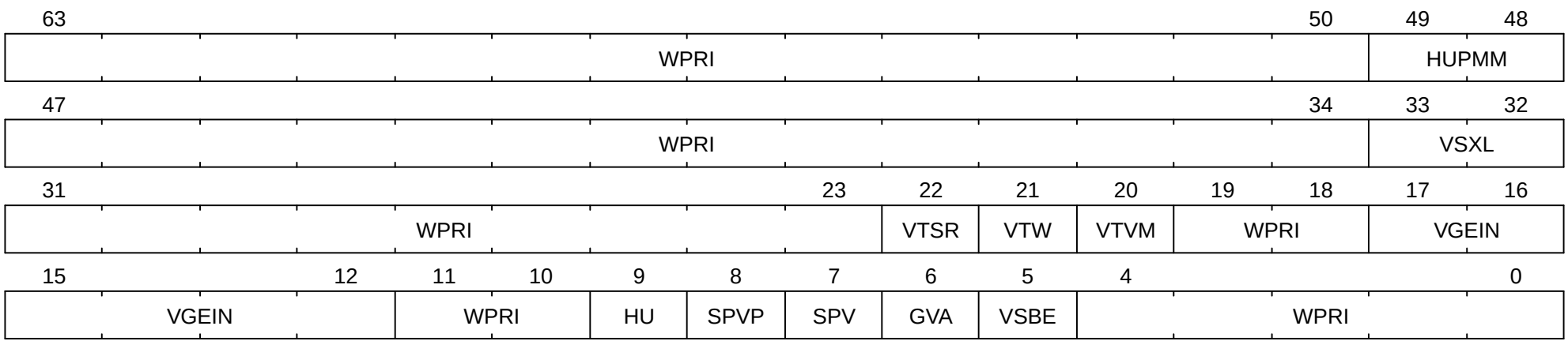
Figure 113. Hypervisor status register ( hstatus ) when HSXLEN =64.
