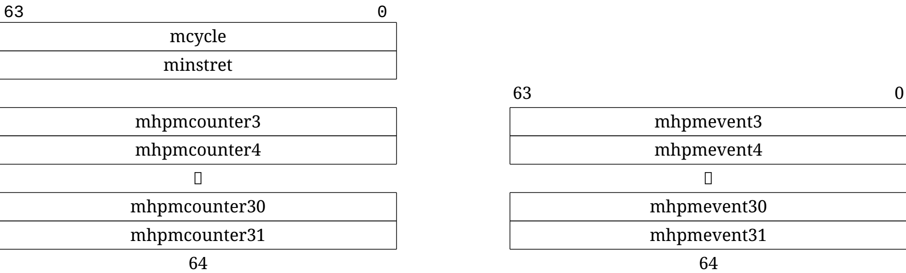
Figure 50. Hardware performance monitor counters.
