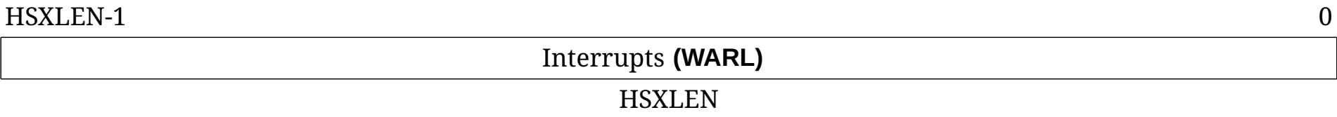
Figure 119. Hypervisor interrupt-enable register ( hie ).
