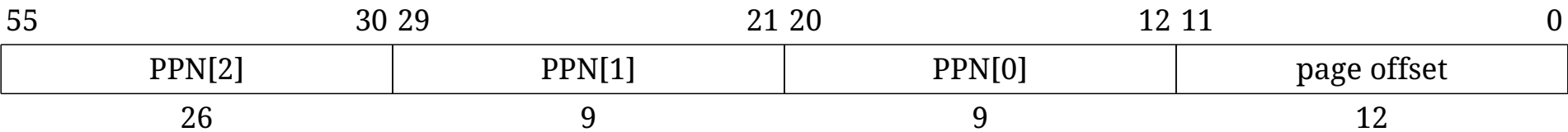
Figure 102. Sv39 physical address.
