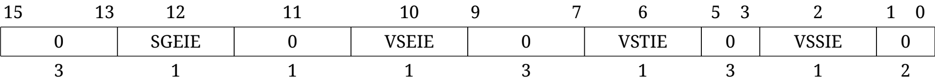
Figure 121. Standard portion (bits 15:0) of hie .
