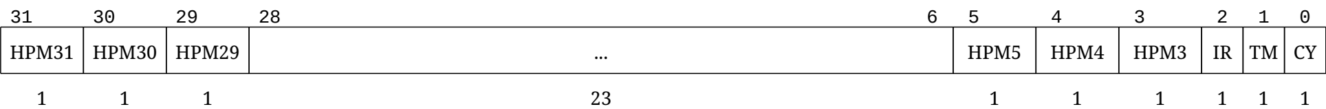
Figure 51. Counter-enable ( mcouneren ) register.
