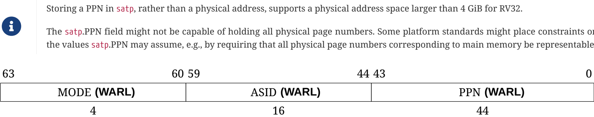
Figure 97. Supervisor address translation and protection (satp) register when SXLEN=64, for MODE values Bare, Sv39, Sv48, and Sv57.
