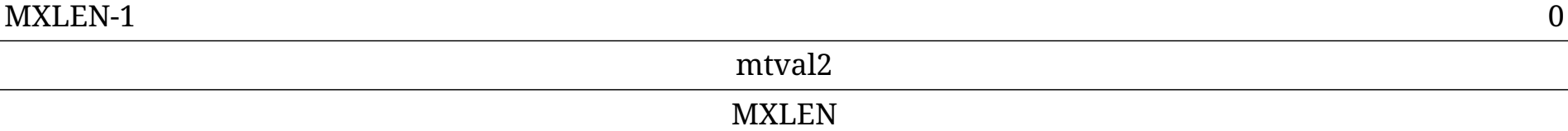
Figure 148. Machine second trap value register (mtval2).
