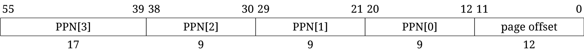
Figure 105. Sv48 physical address.
