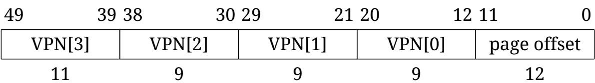
Figure 152. Sv48x4 virtual address (guest physical address).
