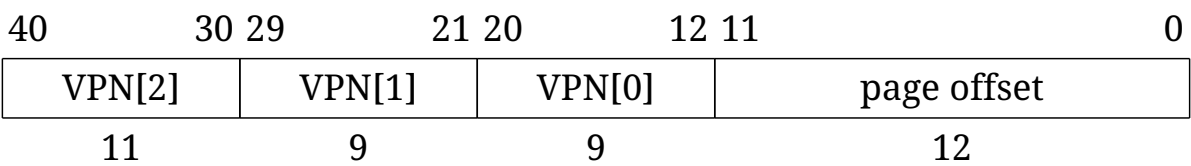
Figure 151. Sv39x4 virtual address (guest physical address).
