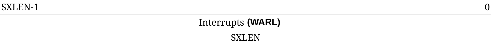
Figure 85. Supervisor interrupt-pending register ( sip ).
