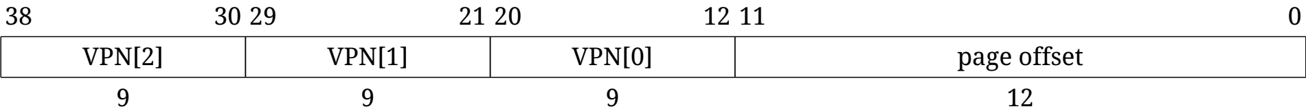
Figure 101. Sv39 virtual address.
