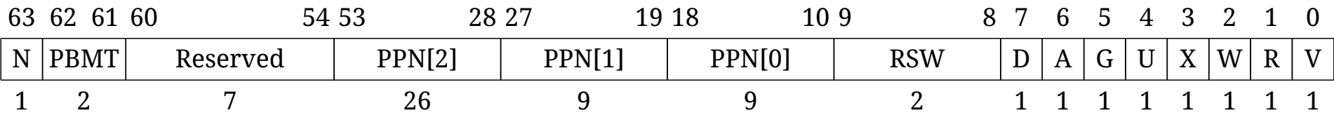
Figure 103. Sv39 page table entry.
