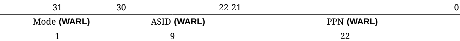
Figure 142. Virtual supervisor address translation and protection vsatp register when VSXLEN=32.
