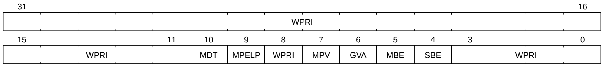
Figure 42. Additional machine-mode status ( mstatush ) register for RV32.
