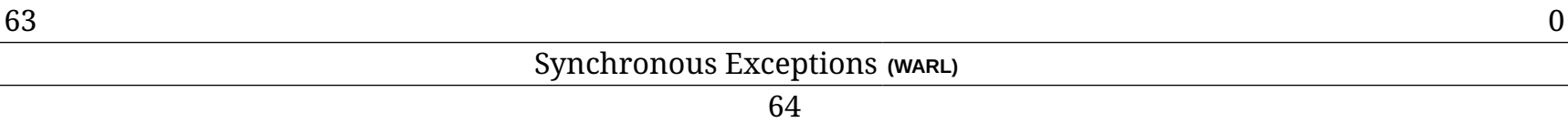
Figure 44. Machine Exception Delegation ( mideleg ) register.
