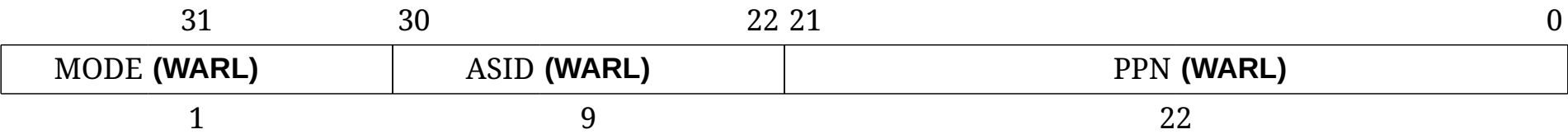
Figure 96. Supervisor address translation and protection (satp) register when SXLEN=32.
