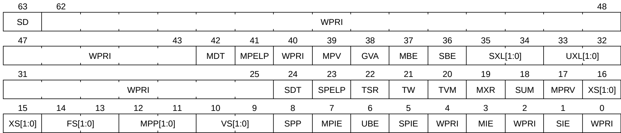
Figure 41. Machine-mode status ( mstatus ) register for RV64
