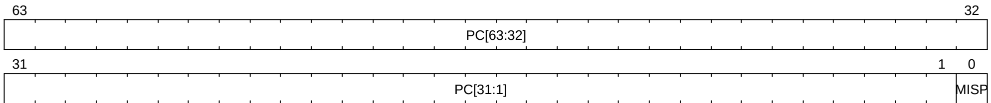
Figure 80. Control Transfer Record Target Register Format for MXLEN=64
