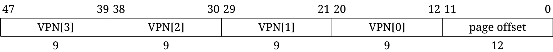
Figure 104. Sv48 virtual address.
