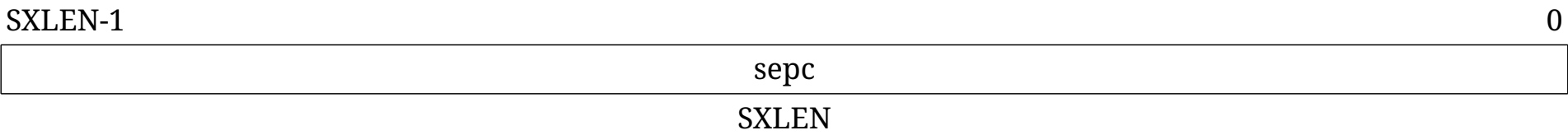
Figure 91. Supervisor exception program counter register.
