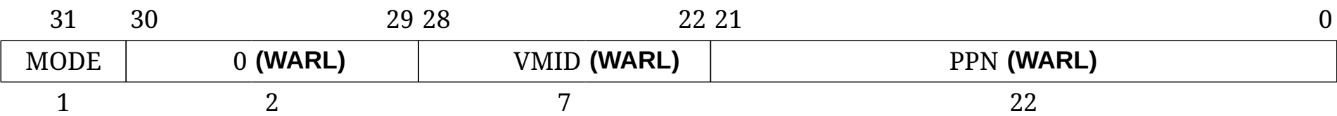
Figure 129. Hypervisor guest address translation and protection register hgap when HSXLEN=32 .
