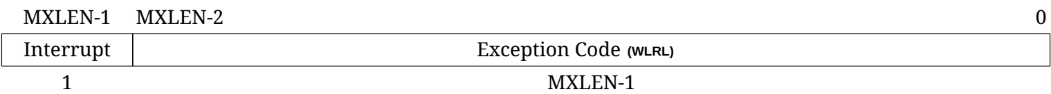
Figure 55. Machine Cause ( mcause ) register.
