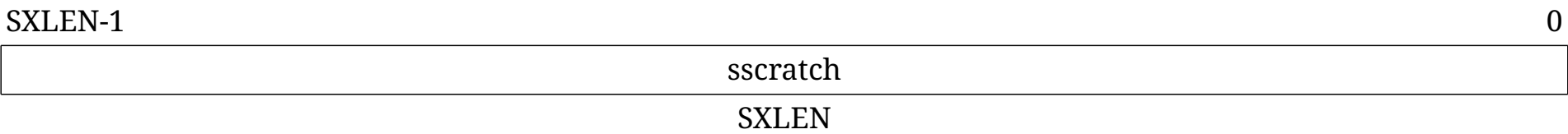
Figure 90. Supervisor Scratch Register
