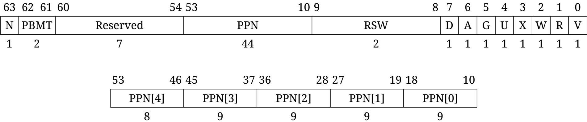
Figure 109. Sv57 page table entry.
