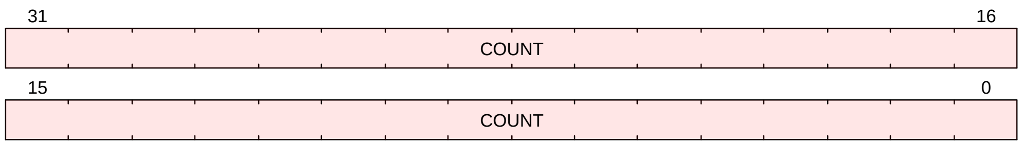
Figure 16. minstreth format
