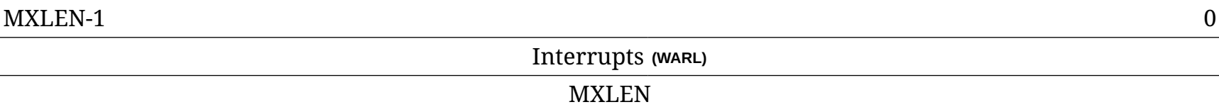
Figure 47. Machine Interrupt-Enable ( mie ) register
