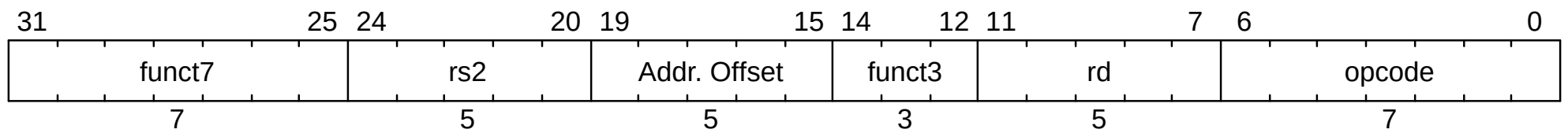
Figure 157. Transformed virtual-machine load/store instruction (HLV, HLVX, HSV). All fields are the same as the trapping instruction except bits 19:15, Addr. Offset
