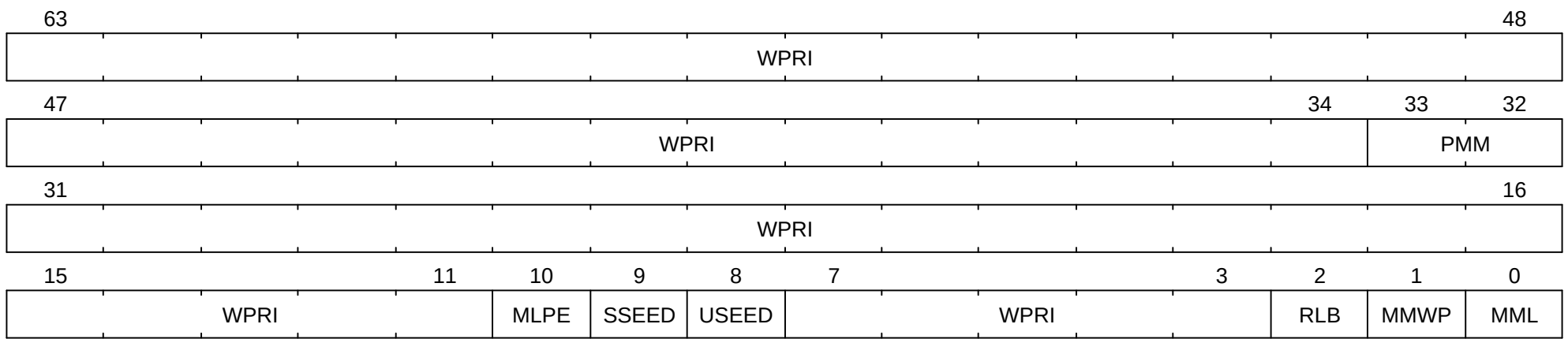
Figure 59. Machine security configuration ( mseccfg ) register.
