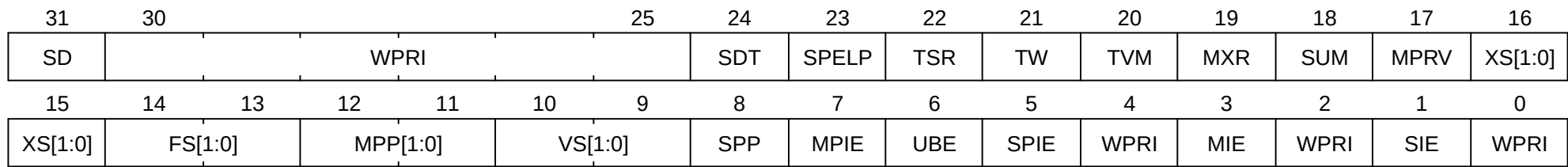
Figure 40. Machine-mode status ( mstatus ) register for RV32
