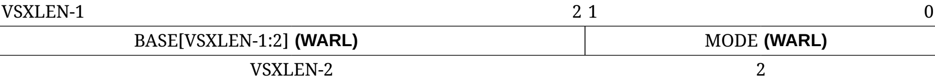
Figure 137. Virtual supervisor trap vector base address register vstvec .
