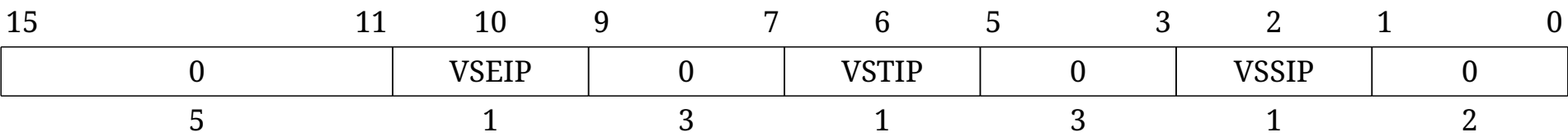
Figure 117. Standard portion (bits 15:0) of hvip .
