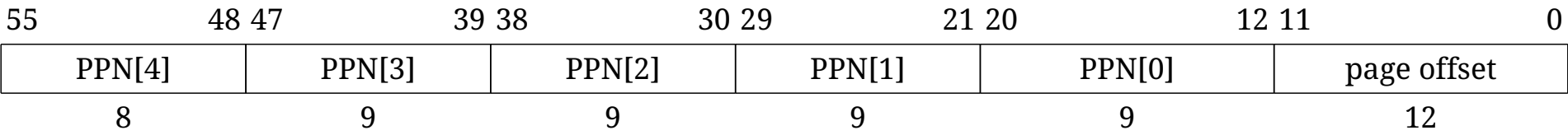
Figure 108. Sv57 physical address.
