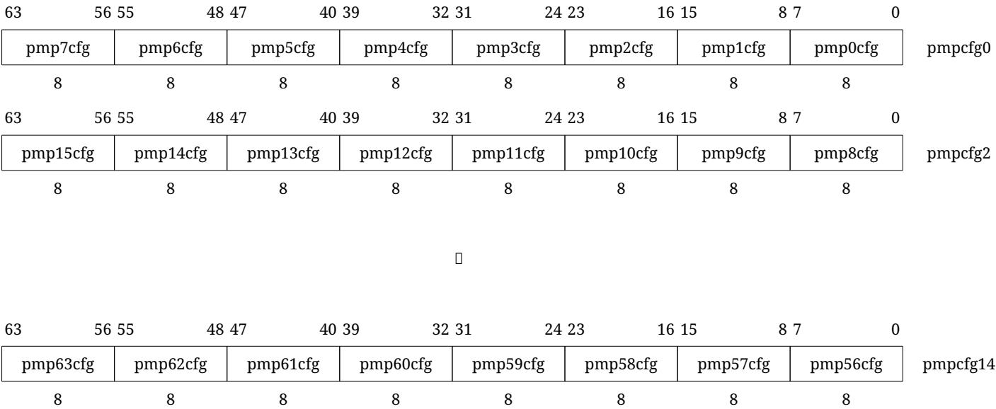
Figure 64. RV64 PMP configuration CSR layout.
