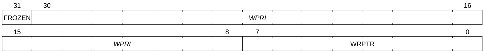
Figure 78. Supervisor Control Transfer Records Status Register Format
