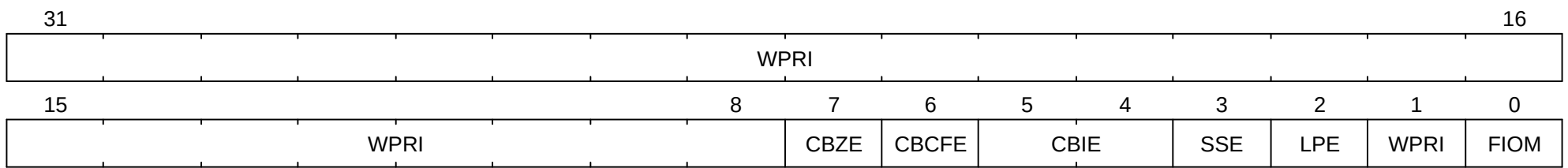
Figure 95. Supervisor environment configuration register ( senvcfg ) for RV32.
