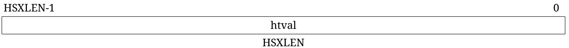
Figure 127. Hypervisor trap value register ( htval ).
