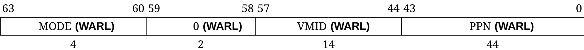
Figure 130. Hypervisor guest address translation and protection register hgap when HSXLEN=64 for MODE values Bare , Sv39x4 , Sv48x4 , and Sv57x4 .
