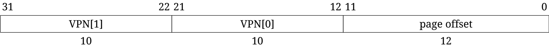
Figure 98. Sv32 virtual address.
