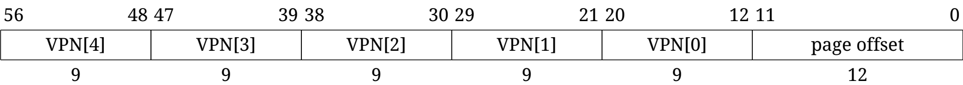
Figure 107. Sv57 virtual address.
