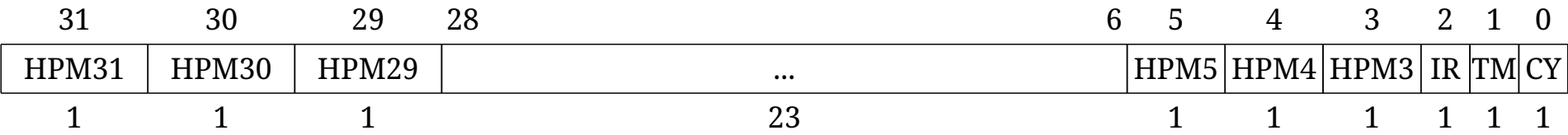
Figure 89. Counter-enable ( scounteren ) register
