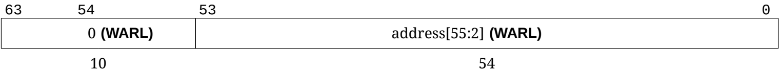
Figure 66. PMP address register format, RV64.
