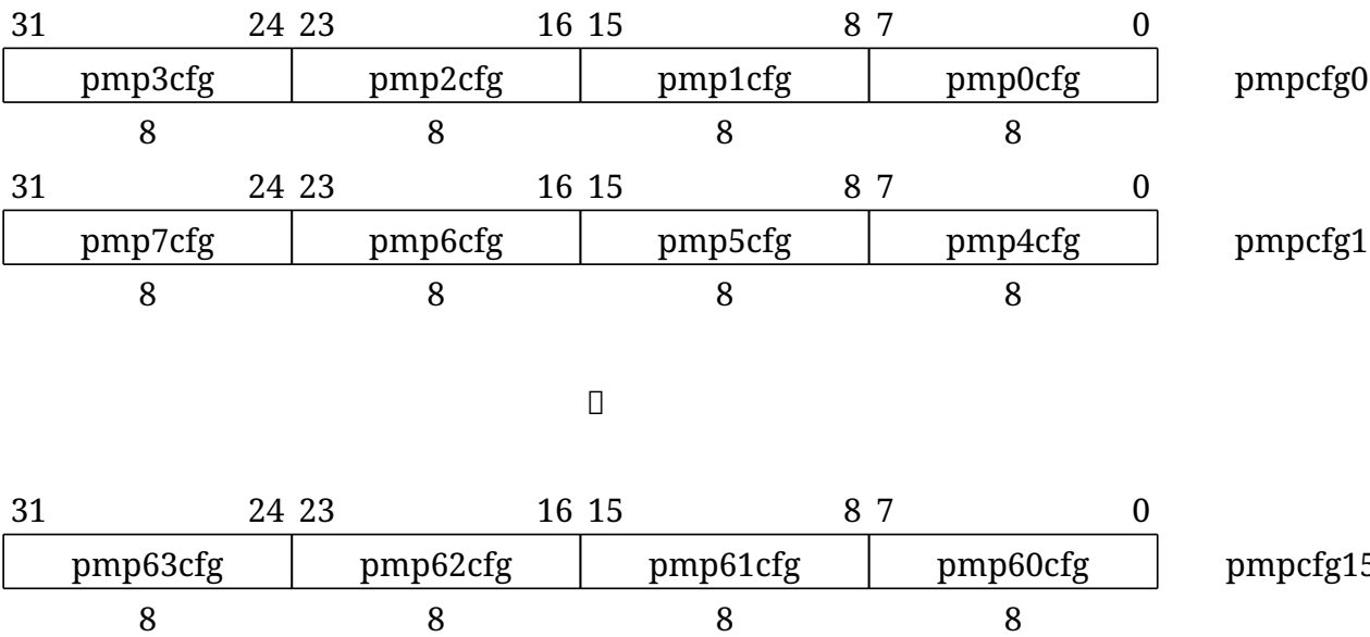
Figure 63. RV32 PMP configuration CSR layout.
