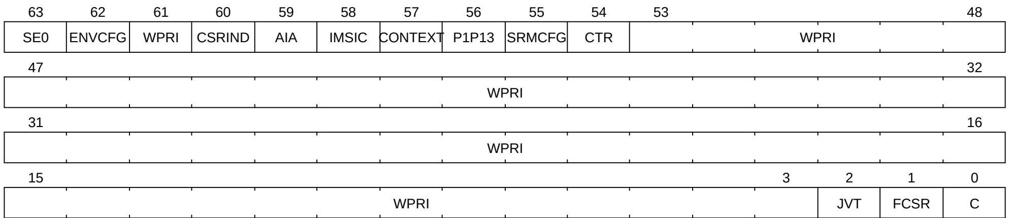
Figure 68. Machine State Enable 0 Register (mstateen0)
