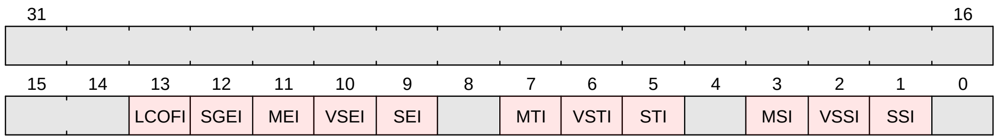
Figure 12. mideleg format
