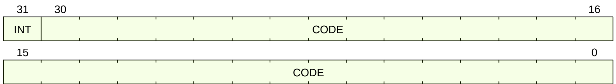
Figure 6. mcause format
