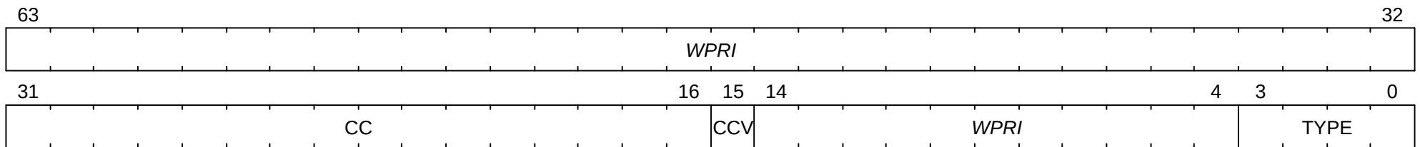
Figure 81. Control Transfer Record Metadata Register Format
