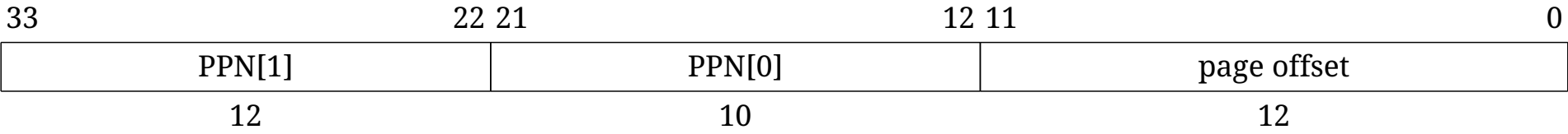
Figure 99. SV32 physical address.
