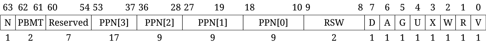
Figure 106. Sv48 page table entry.
