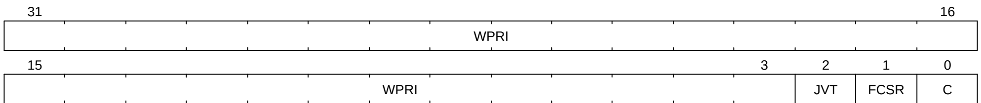
Figure 70. Supervisor State Enable 0 Register (sstateen0)
