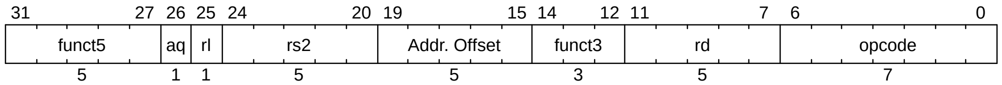
Figure 156. Transformed atomic instruction (load-reserved, store-conditional, or AMO instruction). All fields are the same as the trapping instruction except bits 19:15, Addr. Offset .
