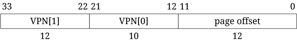
Figure 150. Sv32x4 virtual address (guest physical address).
