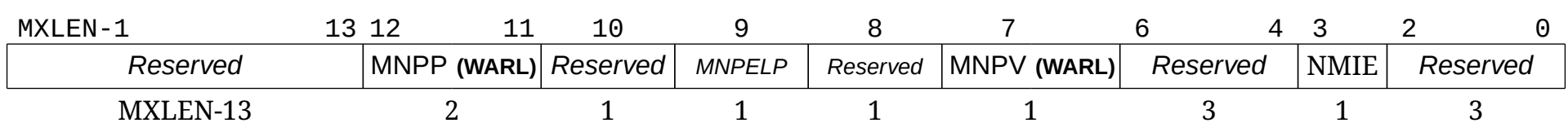
Figure 74. Resumable NMI status register mnstatus .
