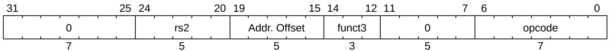
Figure 155. Transformed store instruction (SB, SH, SW, SD, FSW, FSD, FSQ, or FSH). Fields rs2 , funct3 , and opcode are the same as the trapping store instruction.
