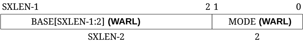
Figure 84. Supervisor trap vector base address ( stvec ) register.
