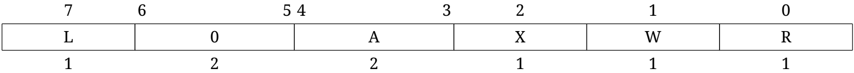
Figure 67. PMP configuration register format.
