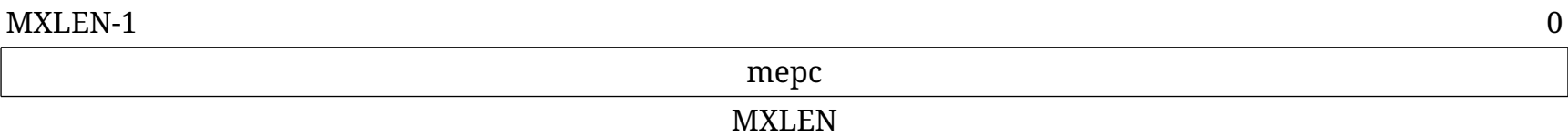
Figure 54. Machine exception program counter register.
