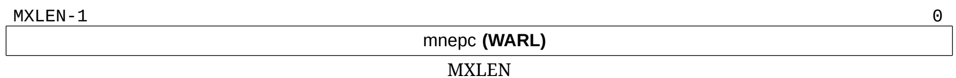
Figure 72. Resumable NMI program counter mnepc .
