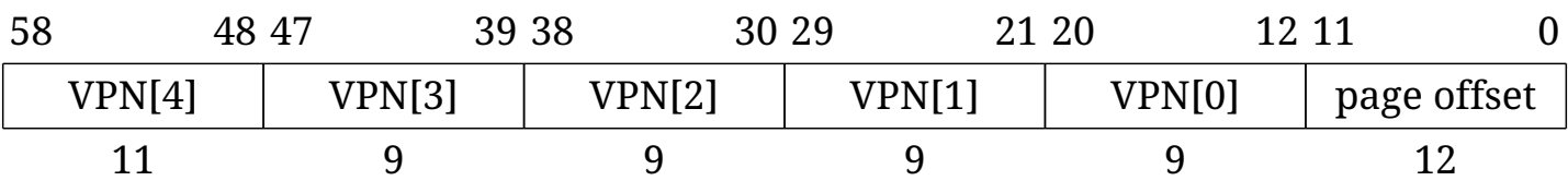
Figure 153. Sv57x4 virtual address (guest physical address).
