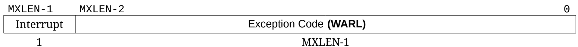
Figure 73. Resumable NMI cause mncause .
