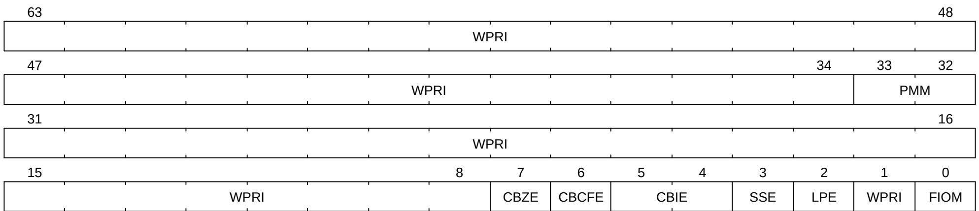
Figure 94. Supervisor environment configuration register ( senvcfg ) for RV64.
