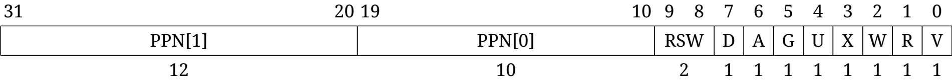
Figure 100. Sv32 page table entry.
