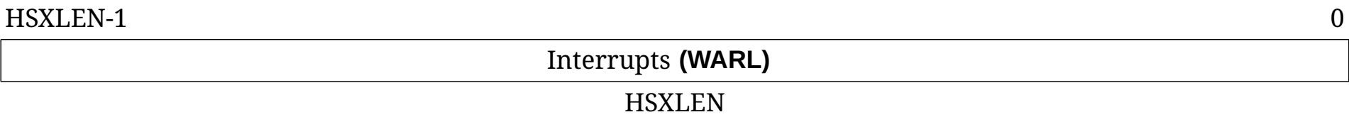
Figure 118. Hypervisor interrupt-pending register ( hip ).
