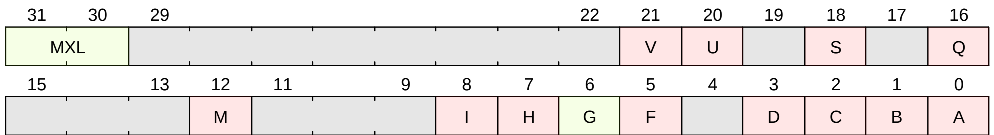
Figure 18. misa format
