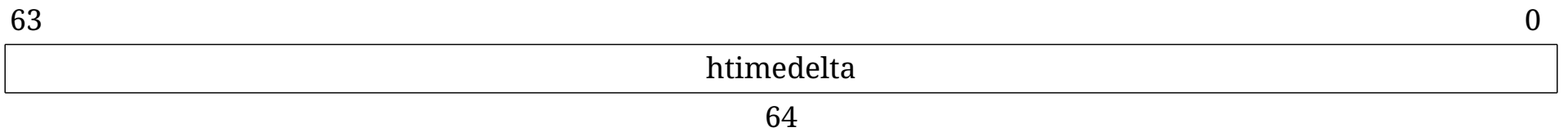
Figure 126. Hypervisor time delta register.
