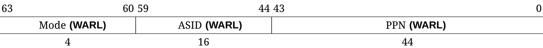
Figure 143. Virtual supervisor address translation and protection vsatp register when VSXLEN=64.
