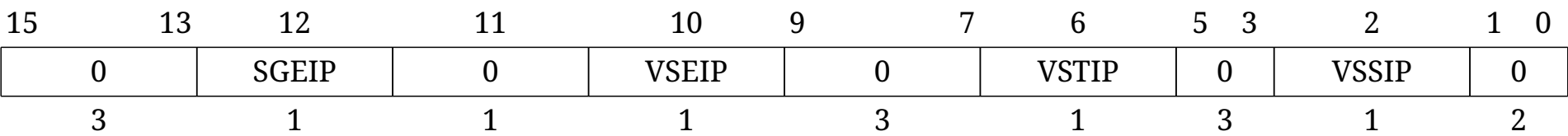
Figure 120. Standard portion (bits 15:0) of hip .
