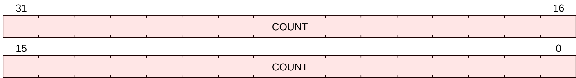
Figure 4. instreth format
