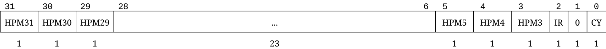
Figure 52. Counter-inhibit mcountinhibit register
