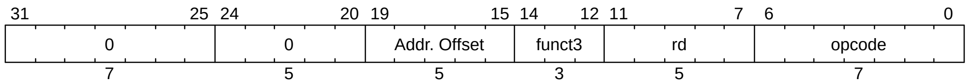
Figure 154. Transformed load instruction (LB, LBU, LH, LHU, LW, LWU, LD, FLW, FLD, FLQ, or FLH). Fields funct3 , rd , and opcode are the same as the trapping load instruction.
