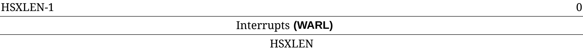
Figure 115. Hypervisor interrupt delegation register (hideleg).
