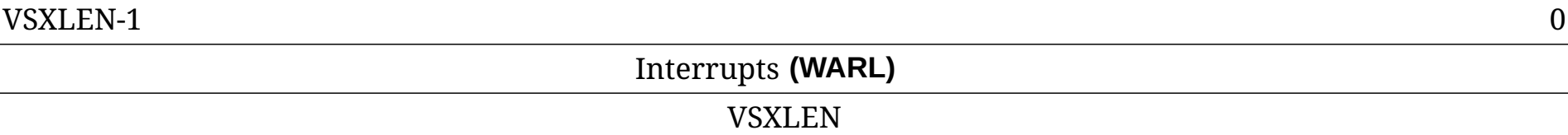
Figure 134. Virtual supervisor interrupt-enable register ( vsie ).
