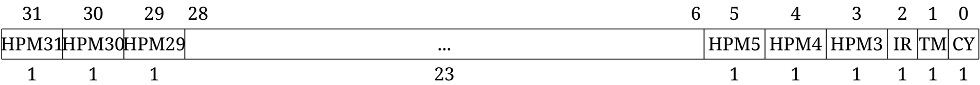
Figure 125. Hypervisor counter-enable register (hcounteren).
