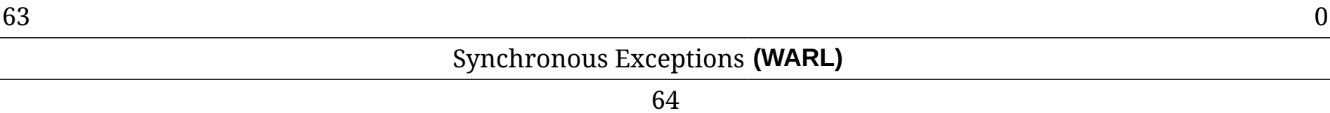
Figure 114. Hypervisor exception delegation register (hedeleg).
