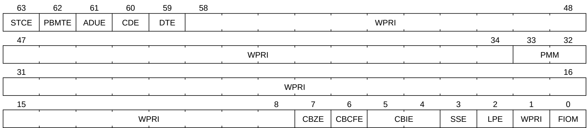
Figure 58. Machine environment configuration ( menvcfg ) register.
