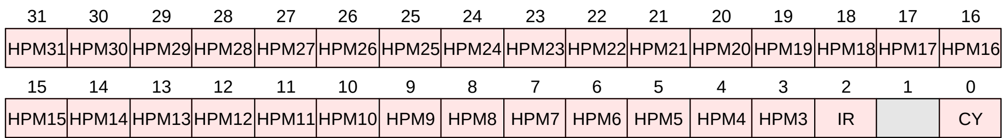
Figure 7. mcountinhibit format
