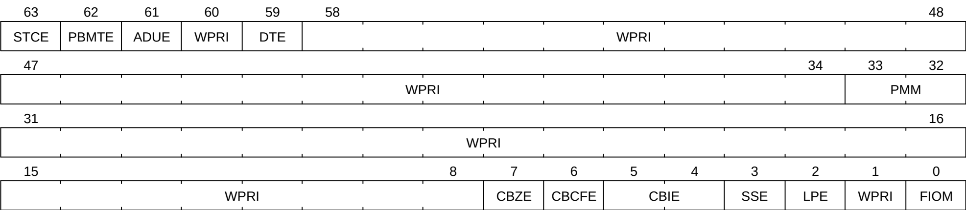
Figure 124. Hypervisor environment configuration register ( henvcfg ).
