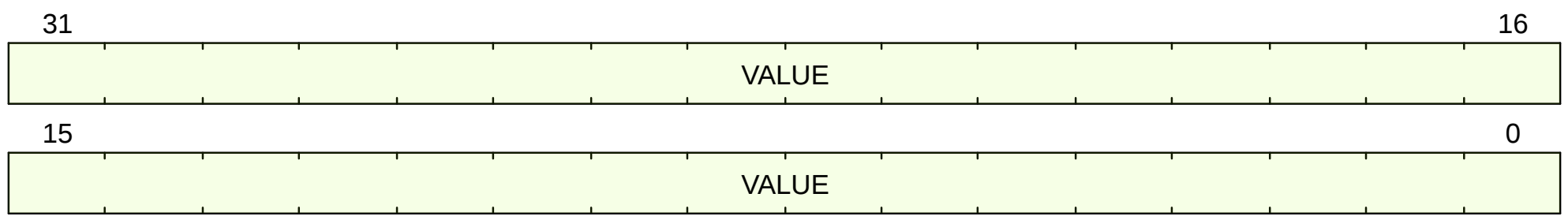
Figure 22. mtval format
