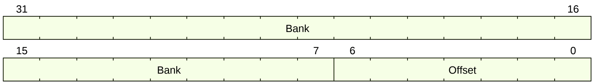
Figure 24. mvendorid format
